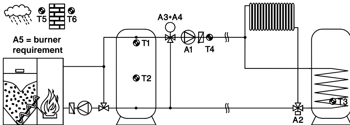
Diagram 128: Buffer tank, heating circuit via pre-mixed district heating pipe, switch-over valve hot water, heating requirement resp. feed pump
