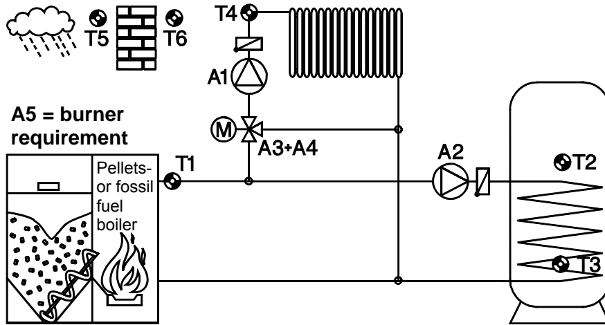
Diagram 16: Automatic boiler, hot water tank, heating circuit, burner requirement
