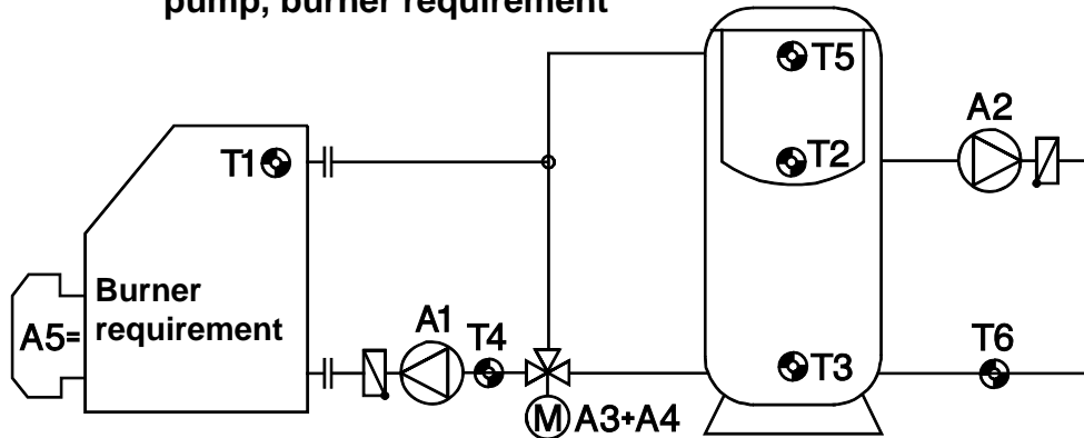
Diagram 144: Automatic boiler, tank, mixer for increasing return, heating circuit pump, burner requirement
