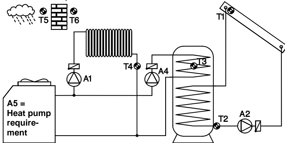
Diagram 112: Heat pump control and requirement, heating circuit pump, solar collector, hot water tank
