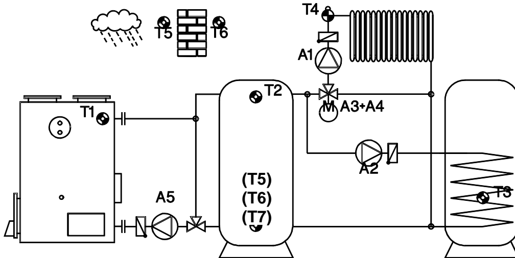
Diagram 64: Solid fuel boiler, buffer, hot water tank, heating circuit
